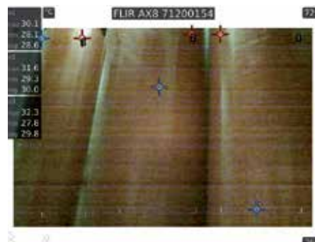
Cast resin transformers need to be able to handle temperature shocks safely. Insulation breakdown on cast resin transformers can lead to system failure and safety issues. The FLIR AX8 can detect temperature raises due to insulation breakdown in an early stage.
